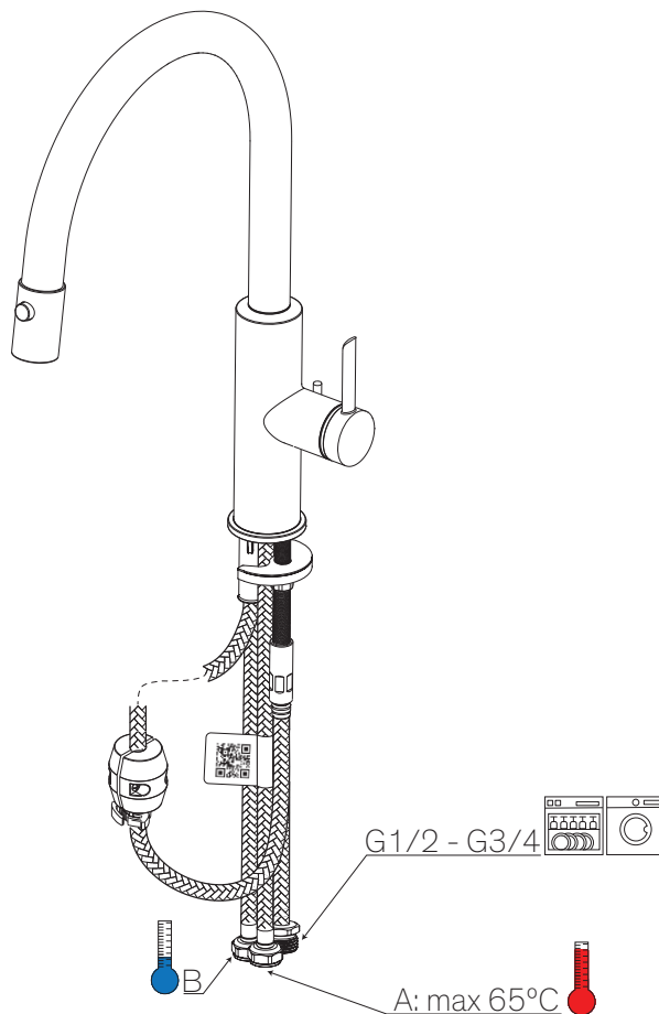
B: With dishwasher shut-off valve
