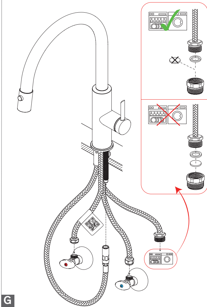
G: With dishwasher shut-off valve
